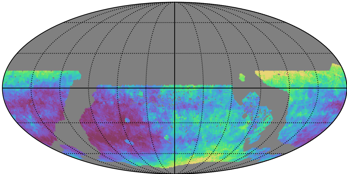
too_ignore_10_1v3.4_10yrs WFD z band: Median seeingEff
