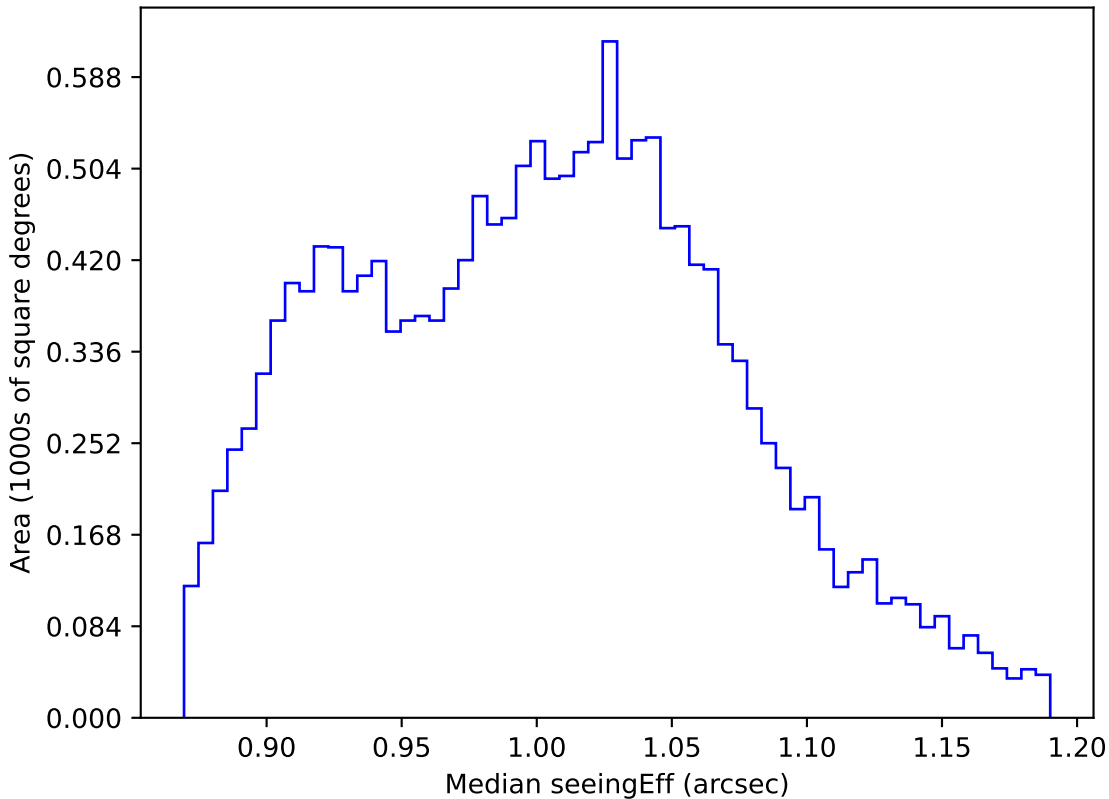
too_ignore_10_1v3.4_10yrs WFD z band: Median seeingEff
