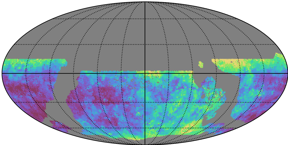
too_ignore_10_1v3.4_10yrs WFD u band: Median seeingEff
