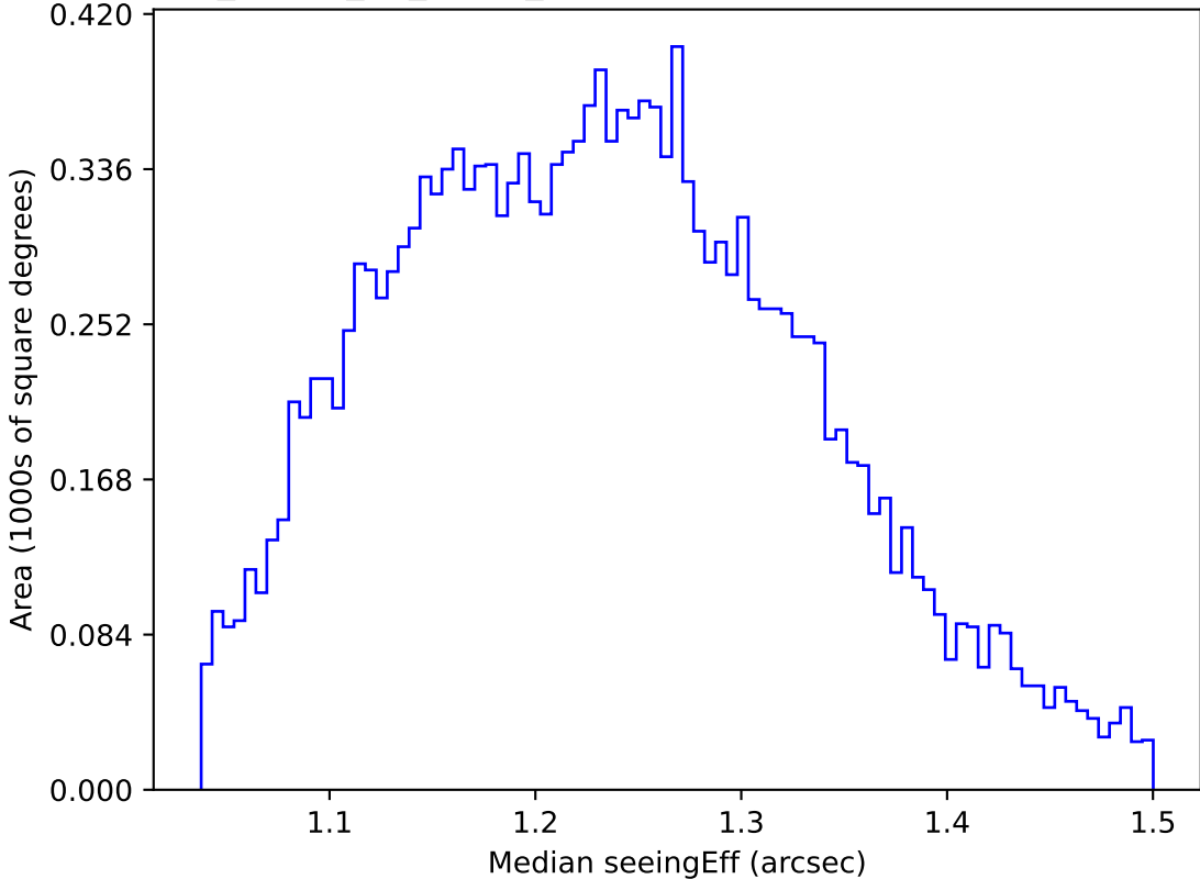
too_ignore_10_1v3.4_10yrs WFD u band: Median seeingEff
