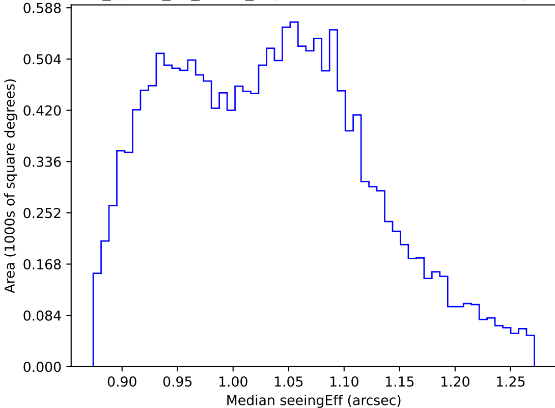
too_ignore_10_1v3.4_10yrs WFD r band: Median seeingEff
