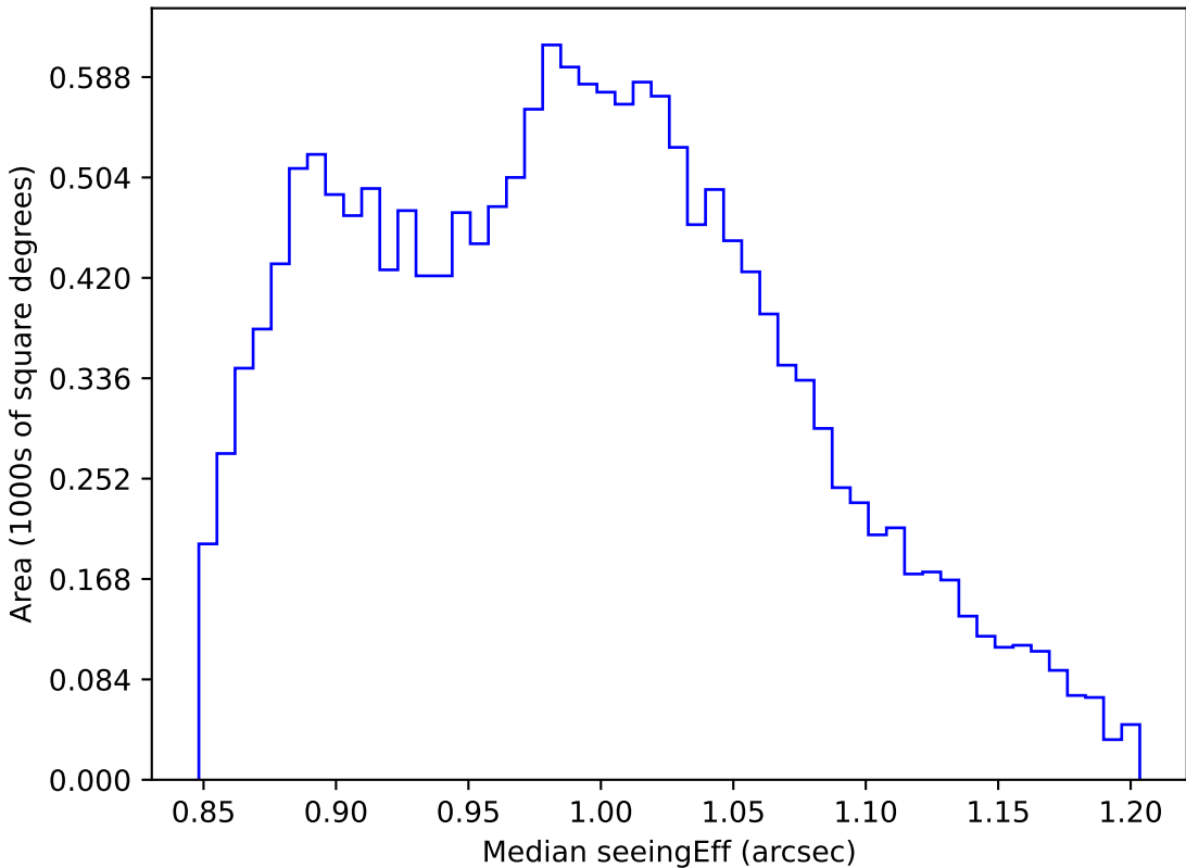
too_ignore_10_1v3.4_10yrs WFD i band: Median seeingEff
