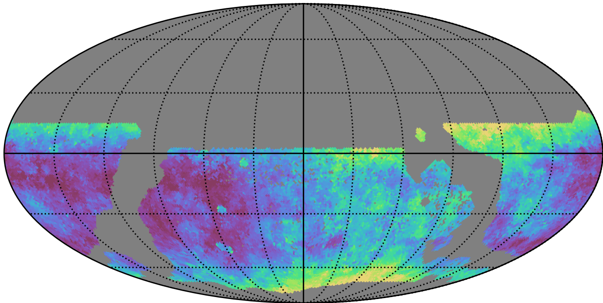
too_ignore_10_1v3.4_10yrs WFD g band: Median seeingEff
