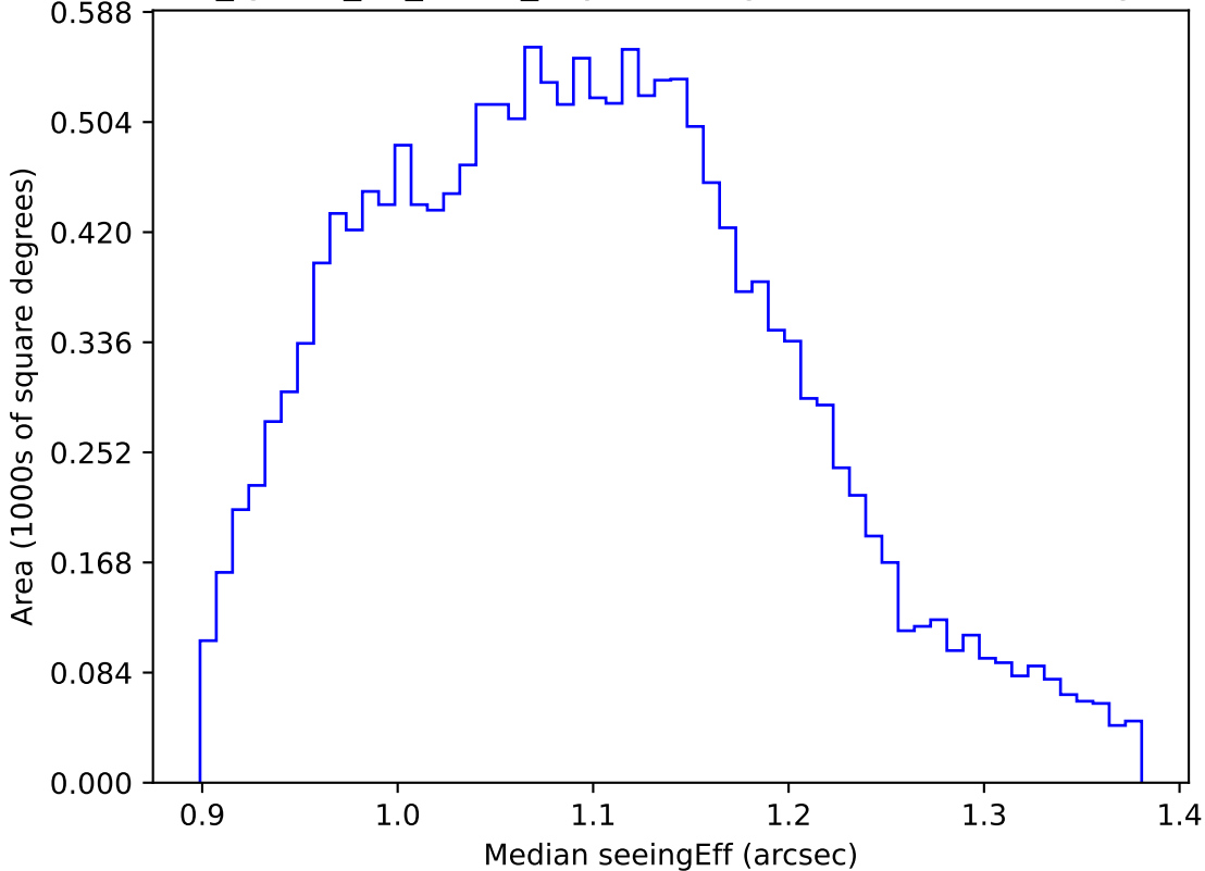
too_ignore_10_1v3.4_10yrs WFD g band: Median seeingEff
