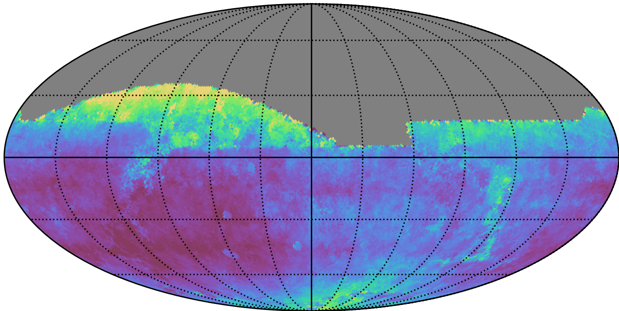
too_ignore_10_1v3.4_10yrs All sky z band: Median seeingEff
