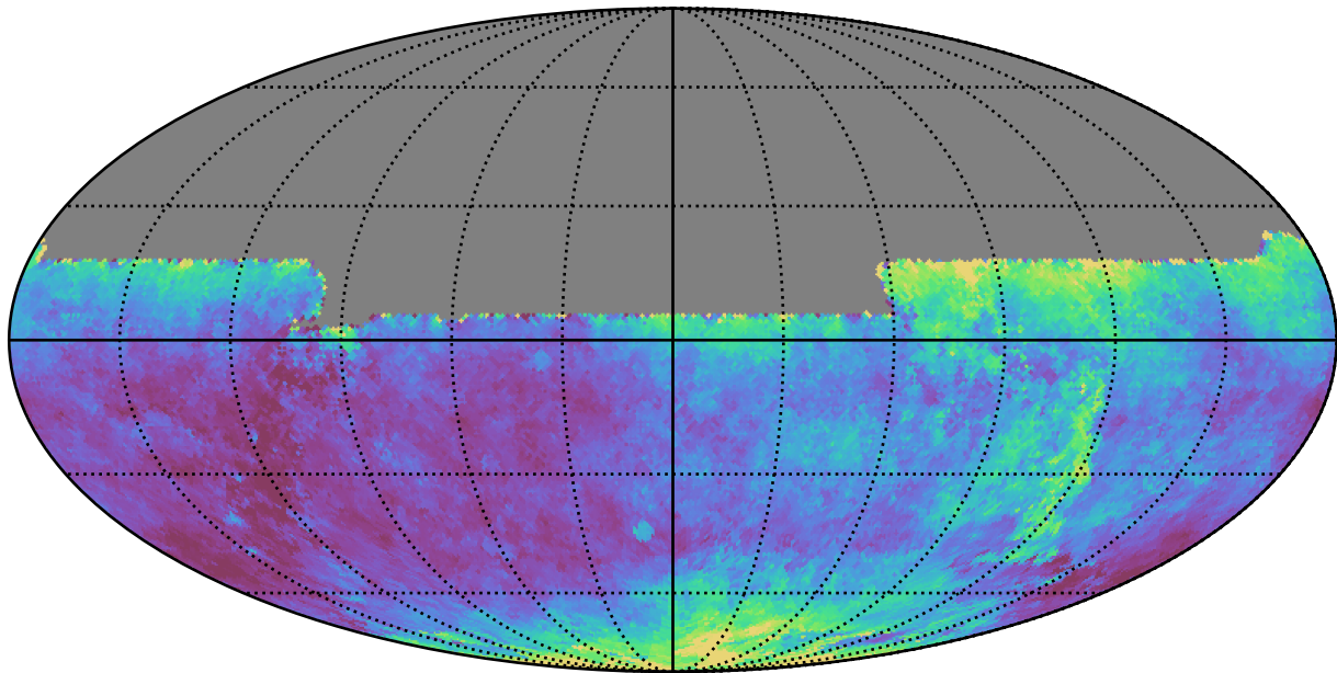
too_ignore_10_1v3.4_10yrs All sky y band: Median seeingEff
