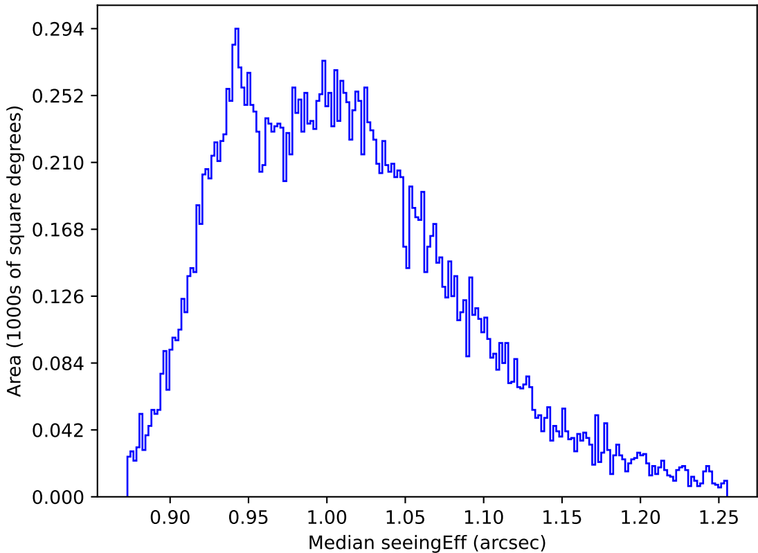
too_ignore_10_1v3.4_10yrs All sky y band: Median seeingEff
