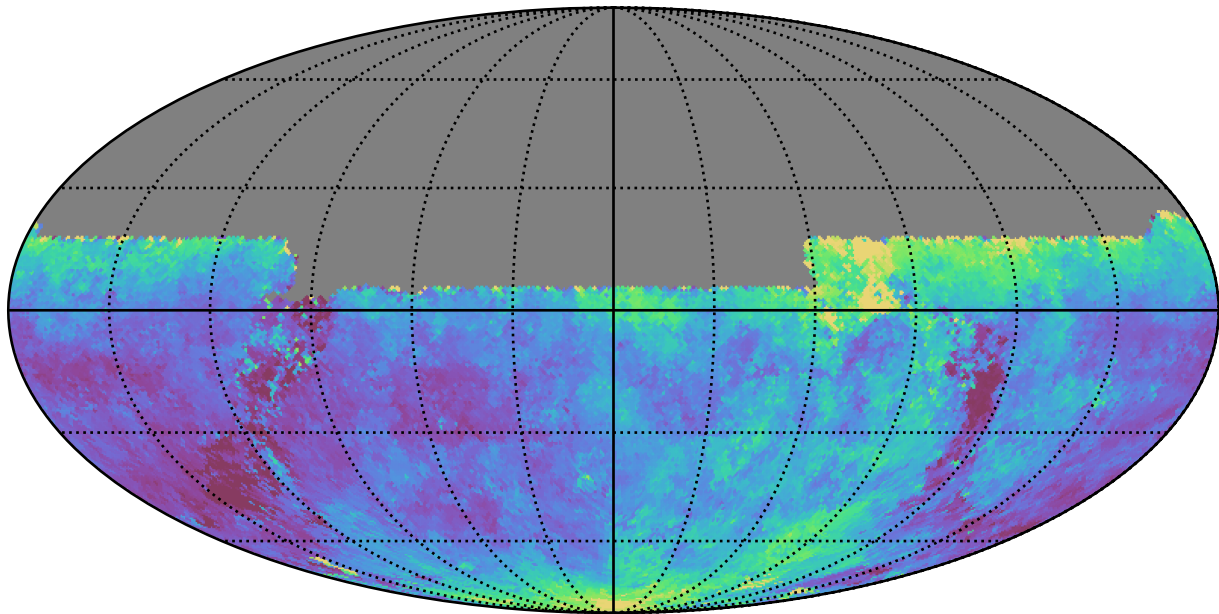
too_ignore_10_1v3.4_10yrs All sky u band: Median seeingEff
