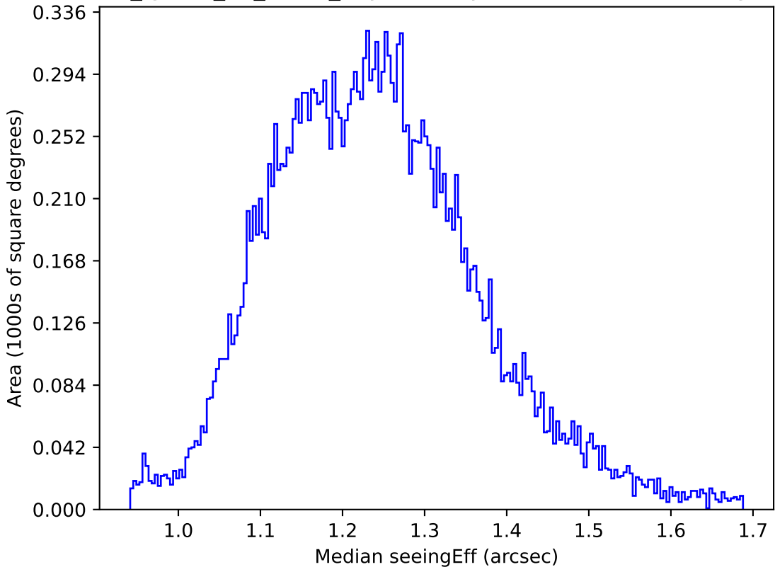
too_ignore_10_1v3.4_10yrs All sky u band: Median seeingEff
