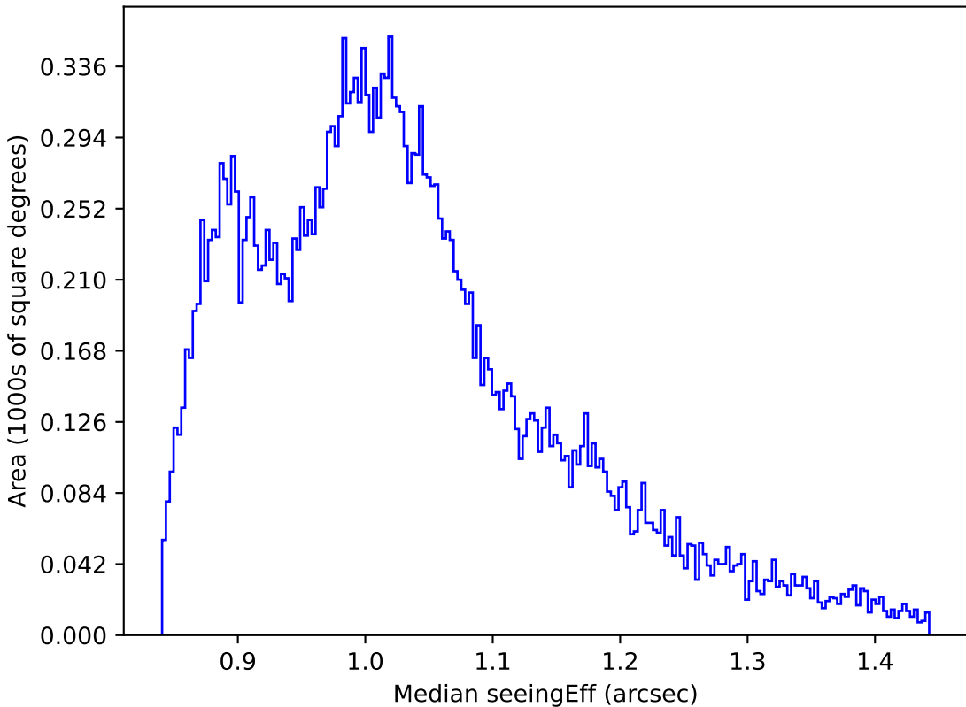
too_ignore_10_1v3.4_10yrs All sky i band: Median seeingEff
