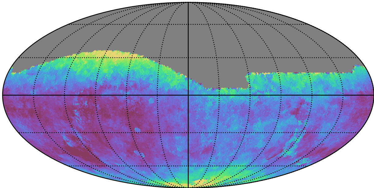
too_ignore_10_1v3.4_10yrs All sky g band: Median seeingEff
