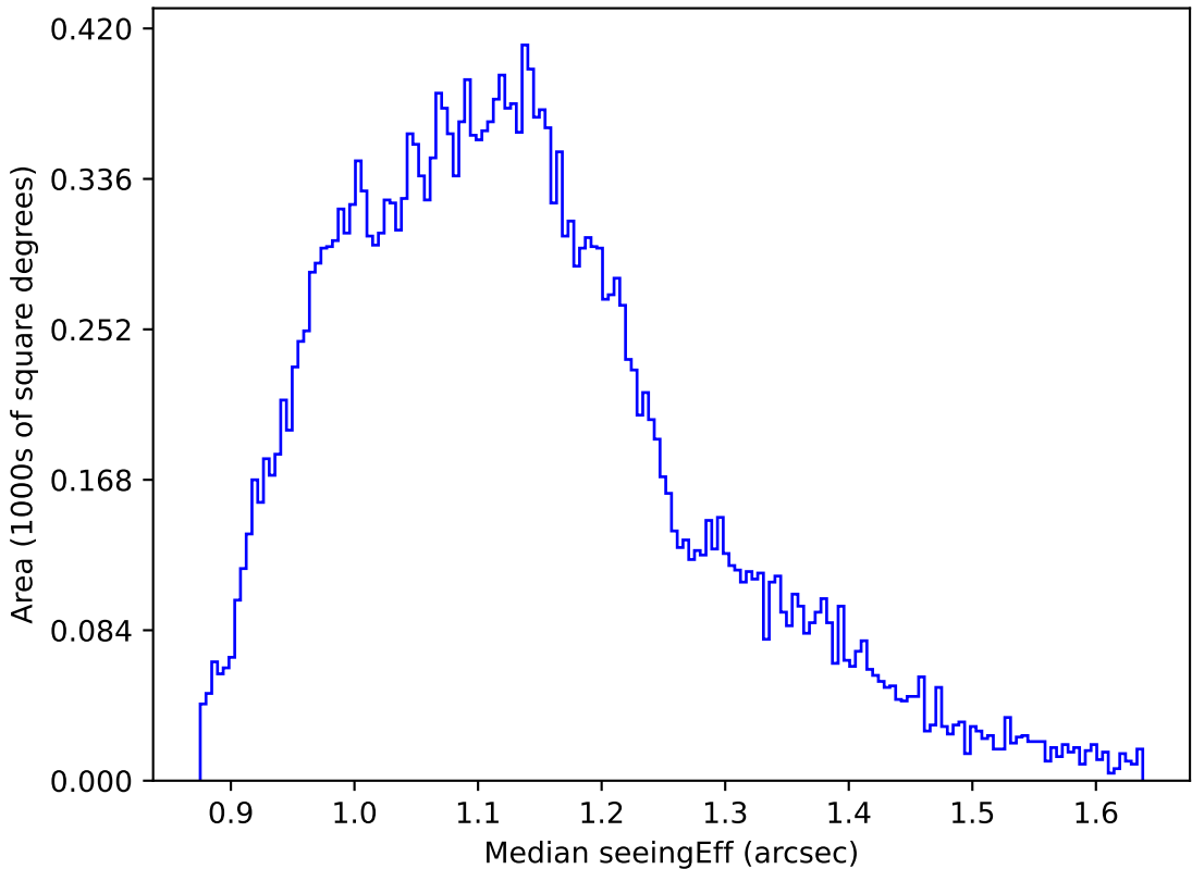
too_ignore_10_1v3.4_10yrs All sky g band: Median seeingEff
