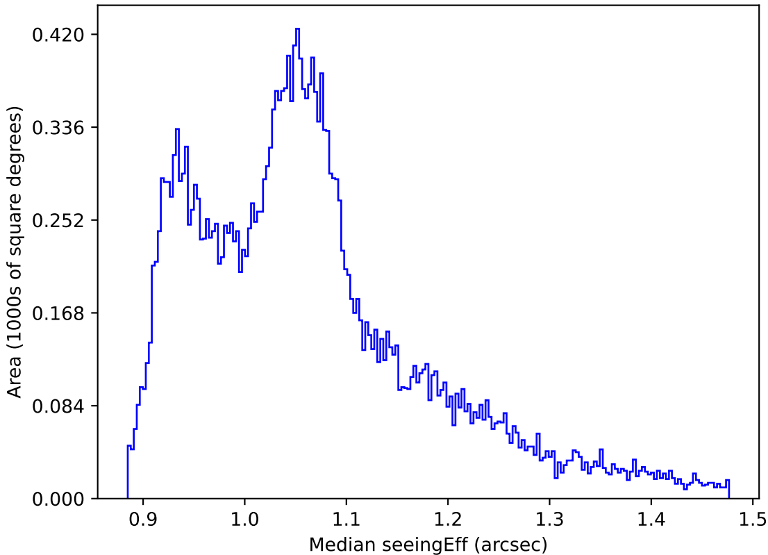
too_ignore_10_1v3.4_10yrs All sky all bands: Median seeingEff
