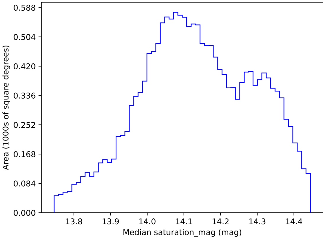
too_ignore_10_1v3.4_10yrs WFD z band: Median saturation_mag
