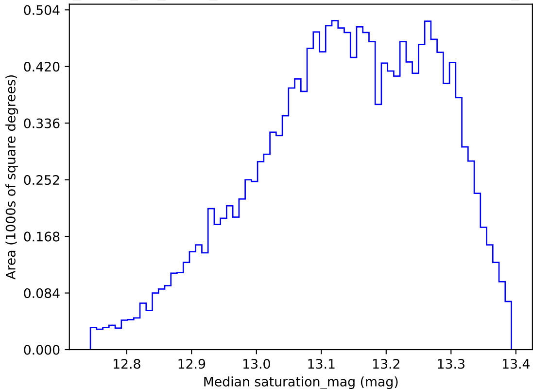
too_ignore_10_1v3.4_10yrs WFD y band: Median saturation_mag
