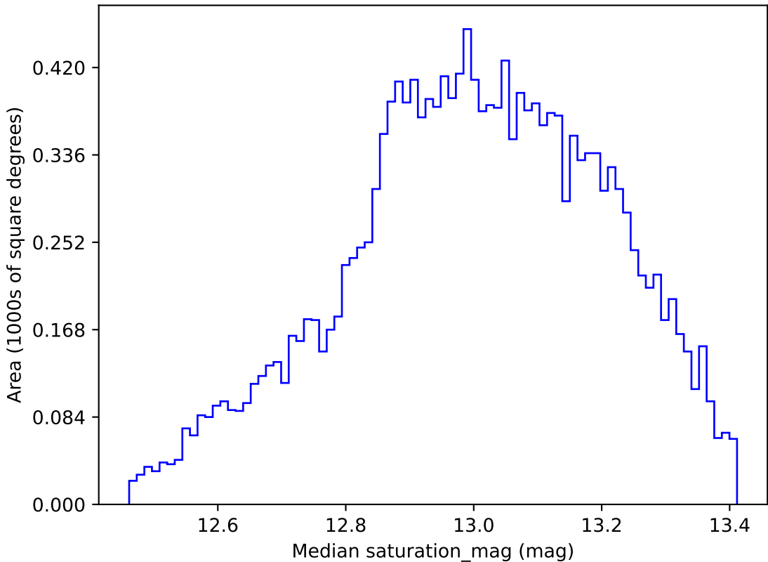
too_ignore_10_1v3.4_10yrs WFD u band: Median saturation_mag
