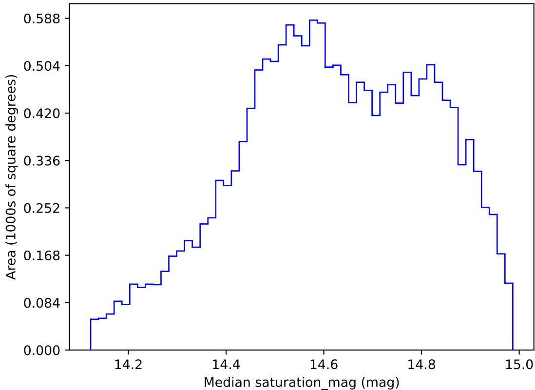
too_ignore_10_1v3.4_10yrs WFD r band: Median saturation_mag
