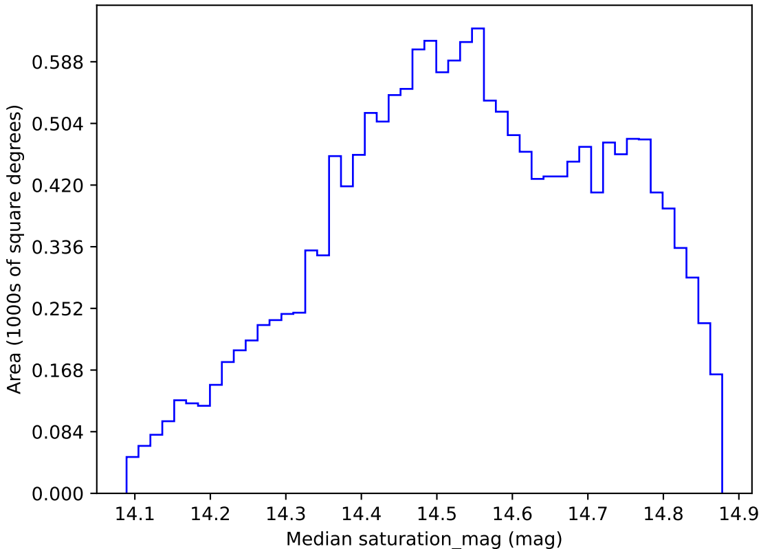
too_ignore_10_1v3.4_10yrs WFD i band: Median saturation_mag
