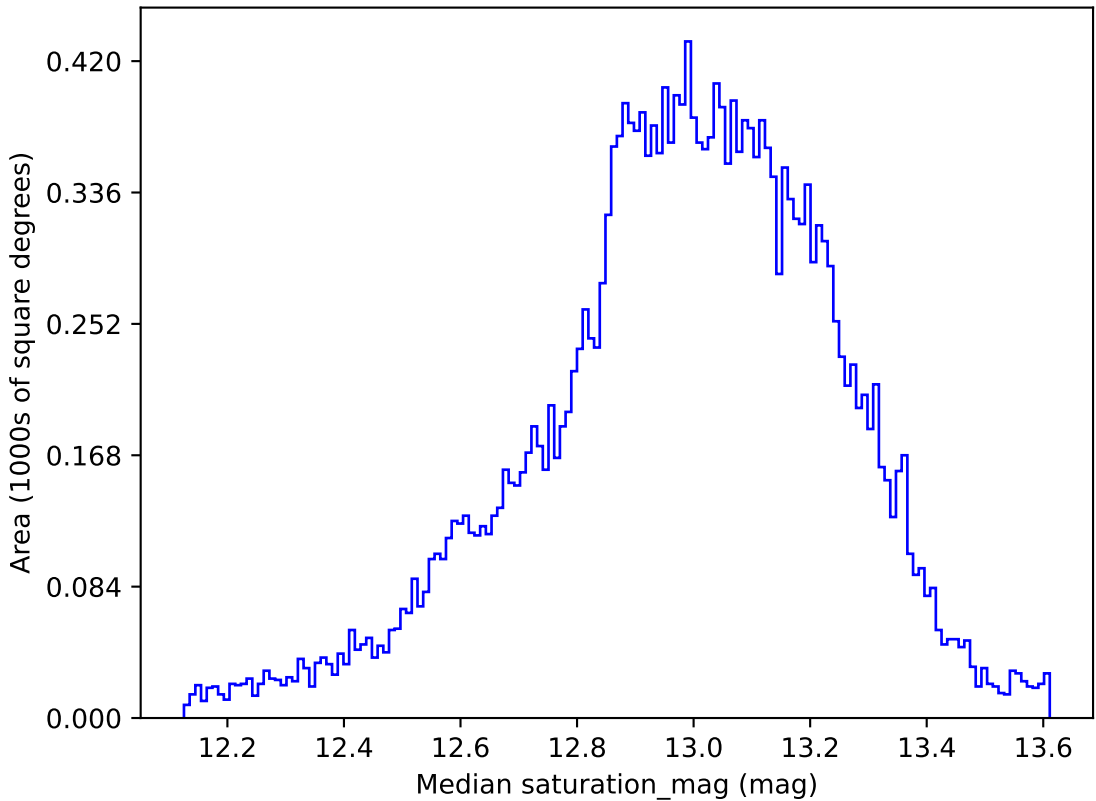
too_ignore_10_1v3.4_10yrs All sky u band: Median saturation_mag
