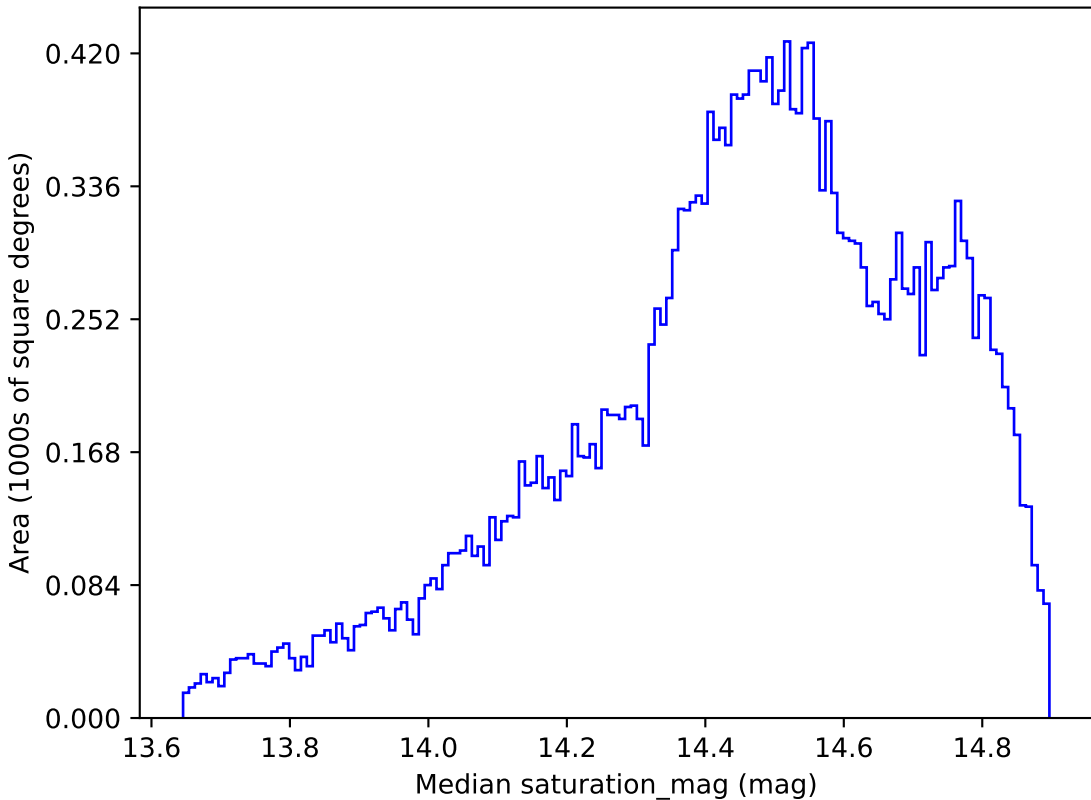
too_ignore_10_1v3.4_10yrs All sky i band: Median saturation_mag
