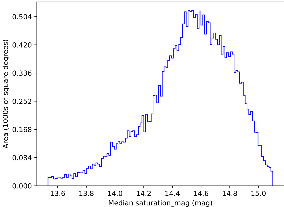
too_ignore_10_1v3.4_10yrs All sky g band: Median saturation_mag
