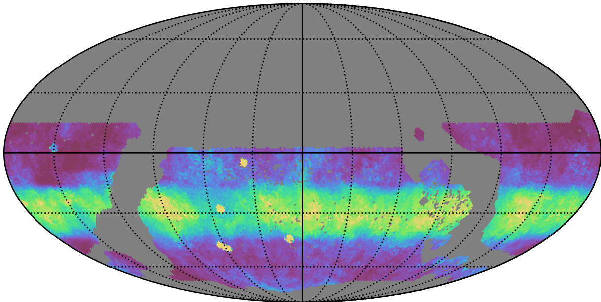
too_ignore_10_1v3.4_10yrs WFD z band: Median normairmass
