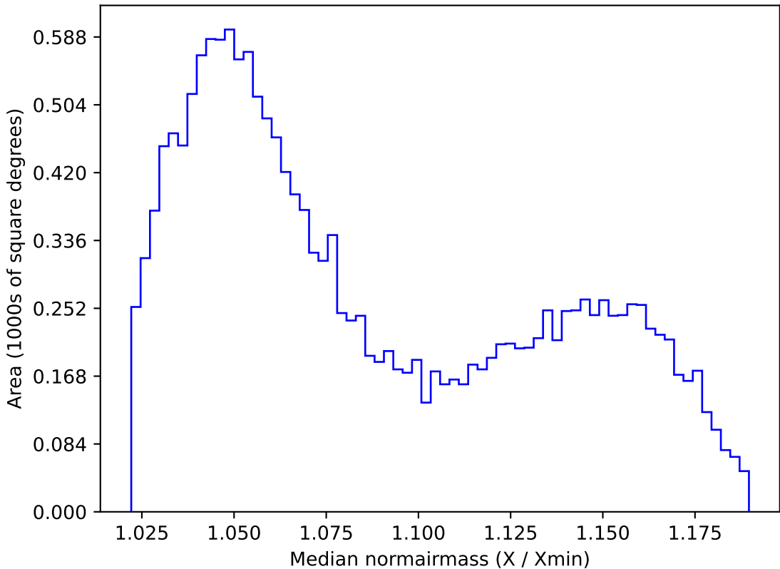
too_ignore_10_1v3.4_10yrs WFD z band: Median normairmass
