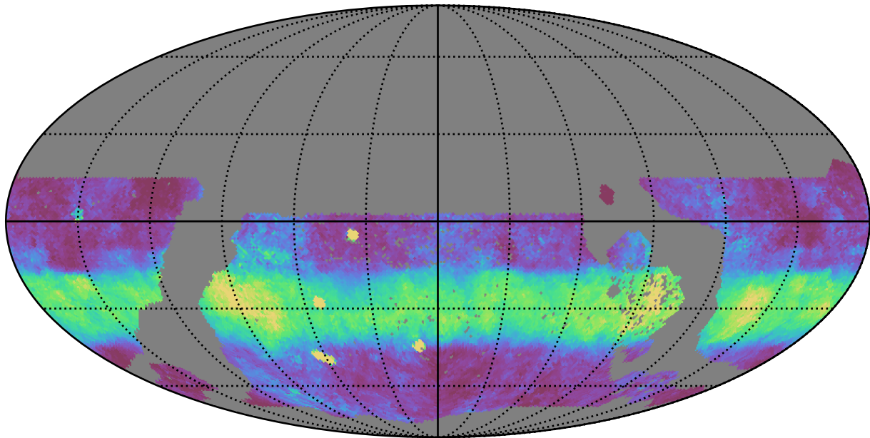
too_ignore_10_1v3.4_10yrs WFD y band: Median normairmass
