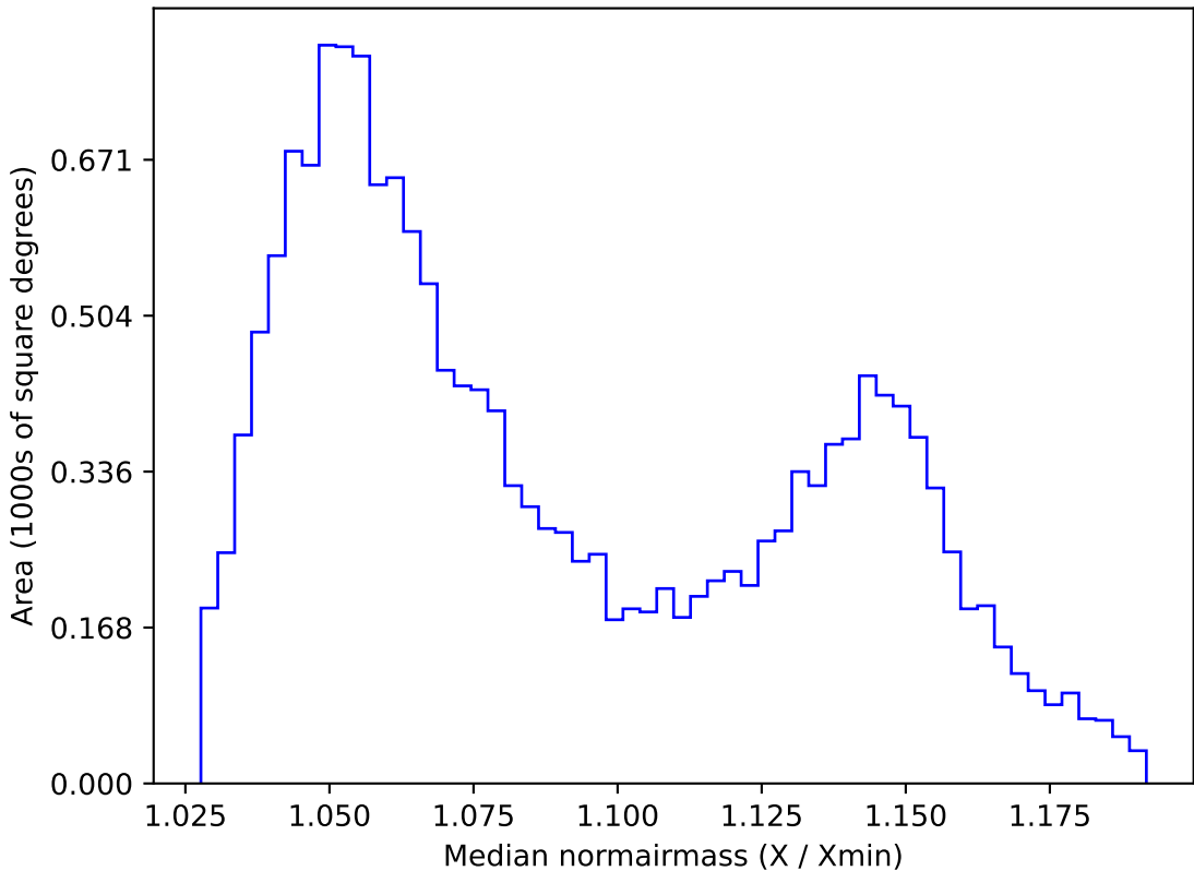
too_ignore_10_1v3.4_10yrs WFD y band: Median normairmass
