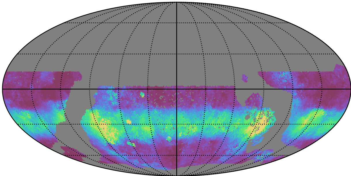
too_ignore_10_1v3.4_10yrs WFD u band: Median normairmass
