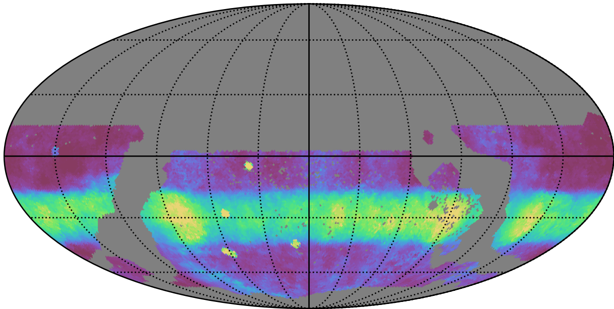
too_ignore_10_1v3.4_10yrs WFD r band: Median normairmass
