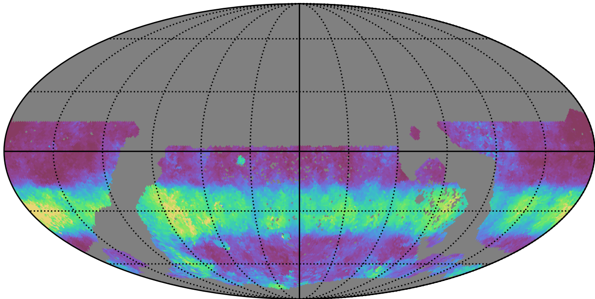
too_ignore_10_1v3.4_10yrs WFD g band: Median normairmass
