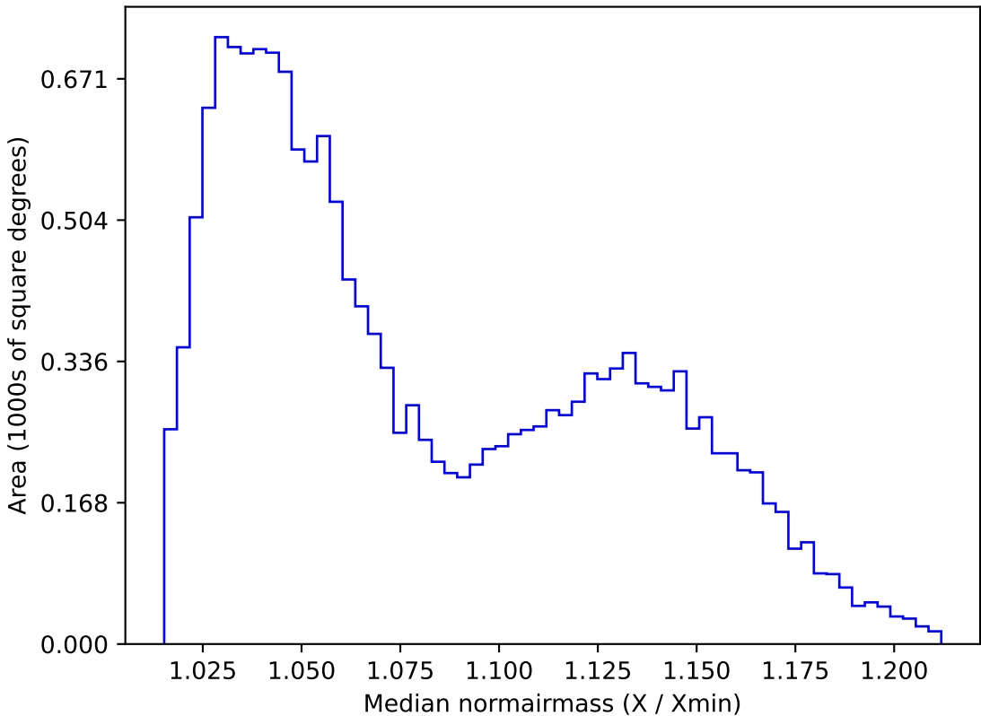
too_ignore_10_1v3.4_10yrs WFD g band: Median normairmass
