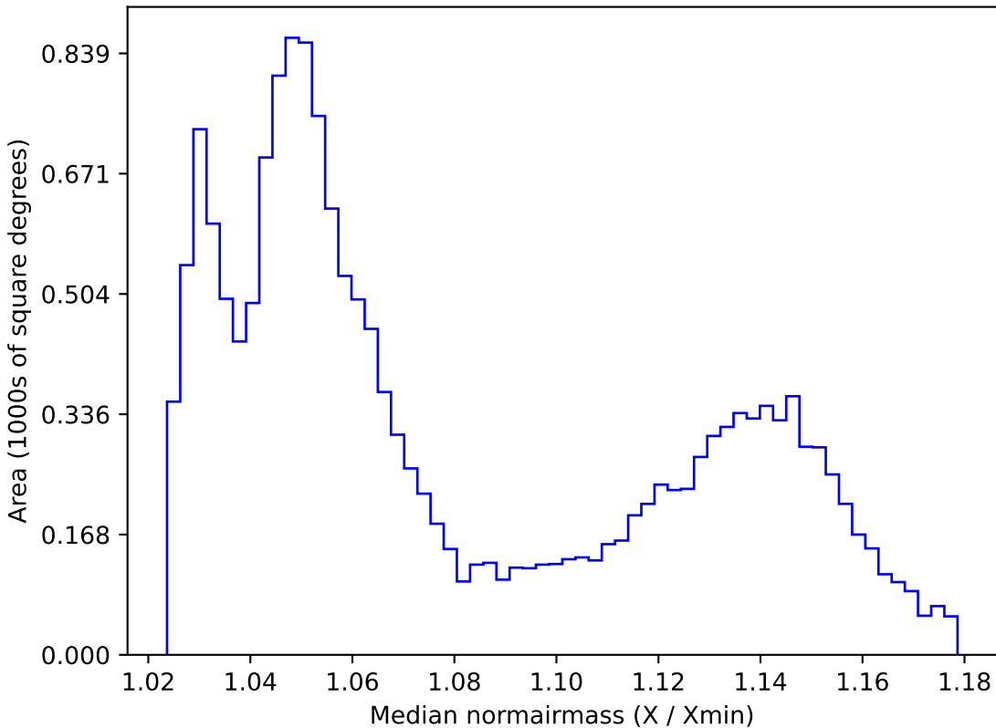
too_ignore_10_1v3.4_10yrs WFD all bands: Median normairmass
