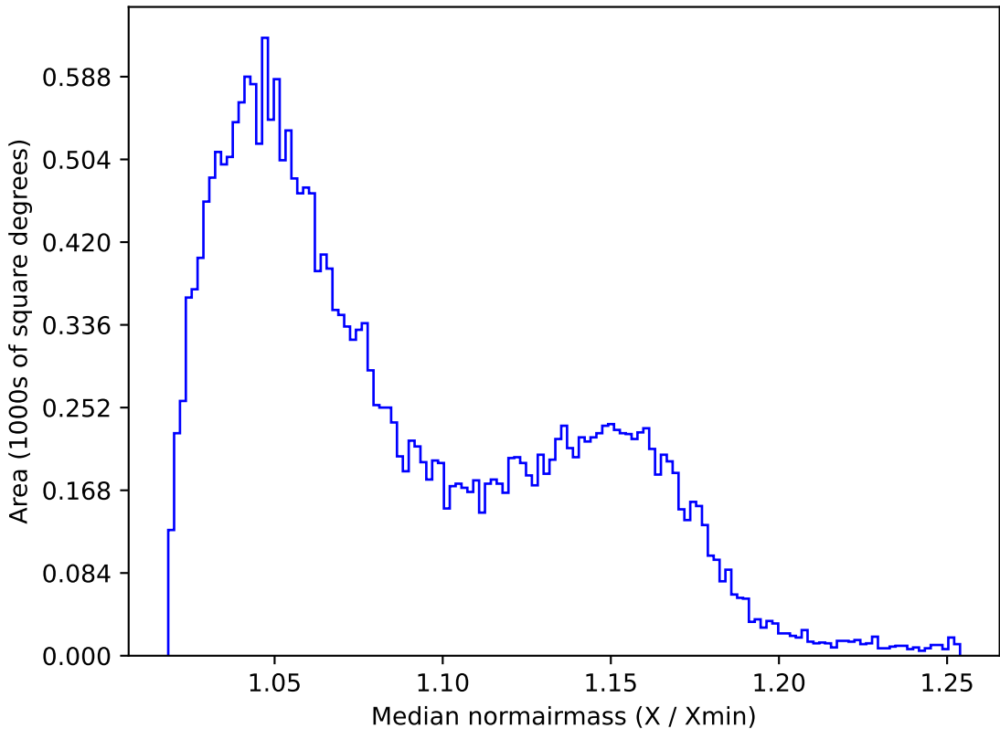
too_ignore_10_1v3.4_10yrs All sky z band: Median normairmass
