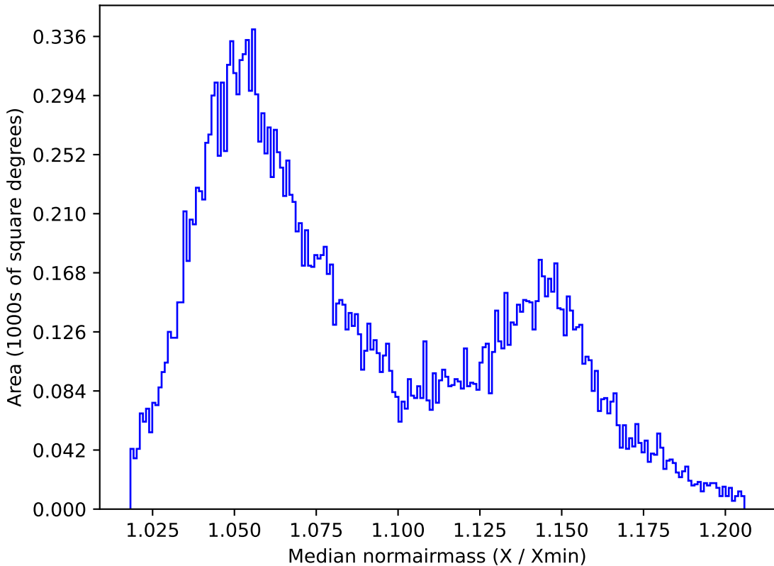
too_ignore_10_1v3.4_10yrs All sky y band: Median normairmass
