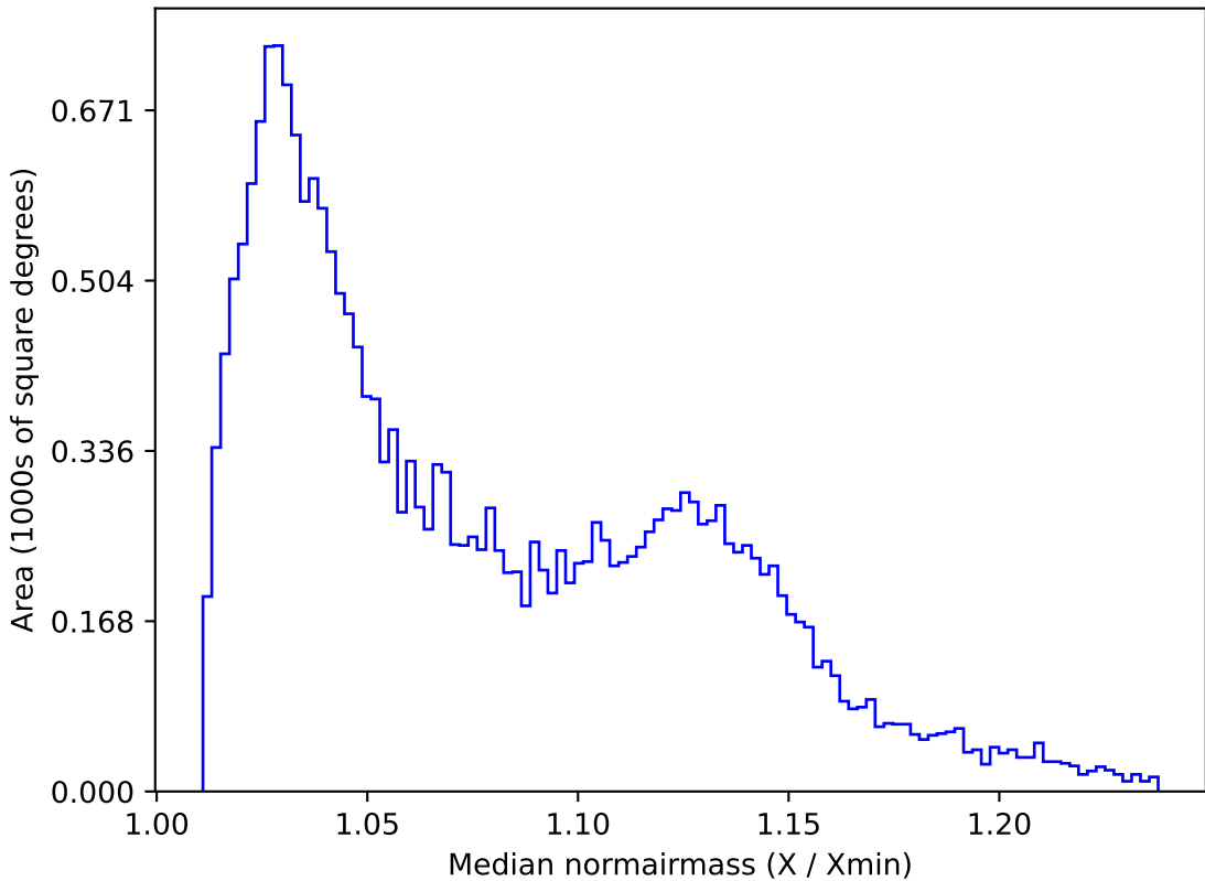
too_ignore_10_1v3.4_10yrs All sky u band: Median normairmass
