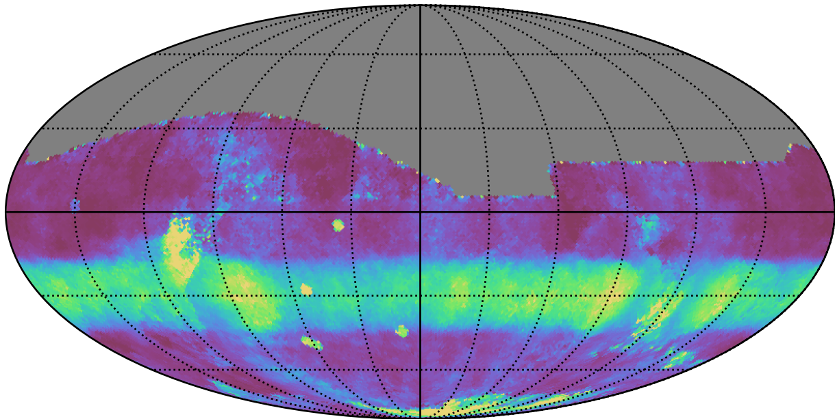
too_ignore_10_1v3.4_10yrs All sky r band: Median normairmass
