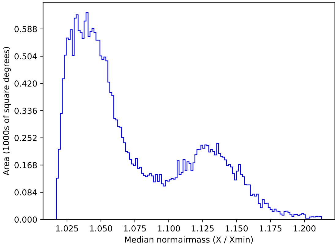
too_ignore_10_1v3.4_10yrs All sky i band: Median normairmass
