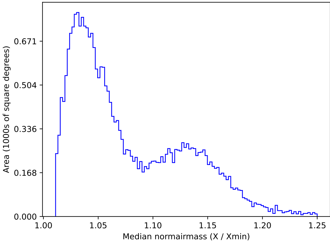
too_ignore_10_1v3.4_10yrs All sky g band: Median normairmass
