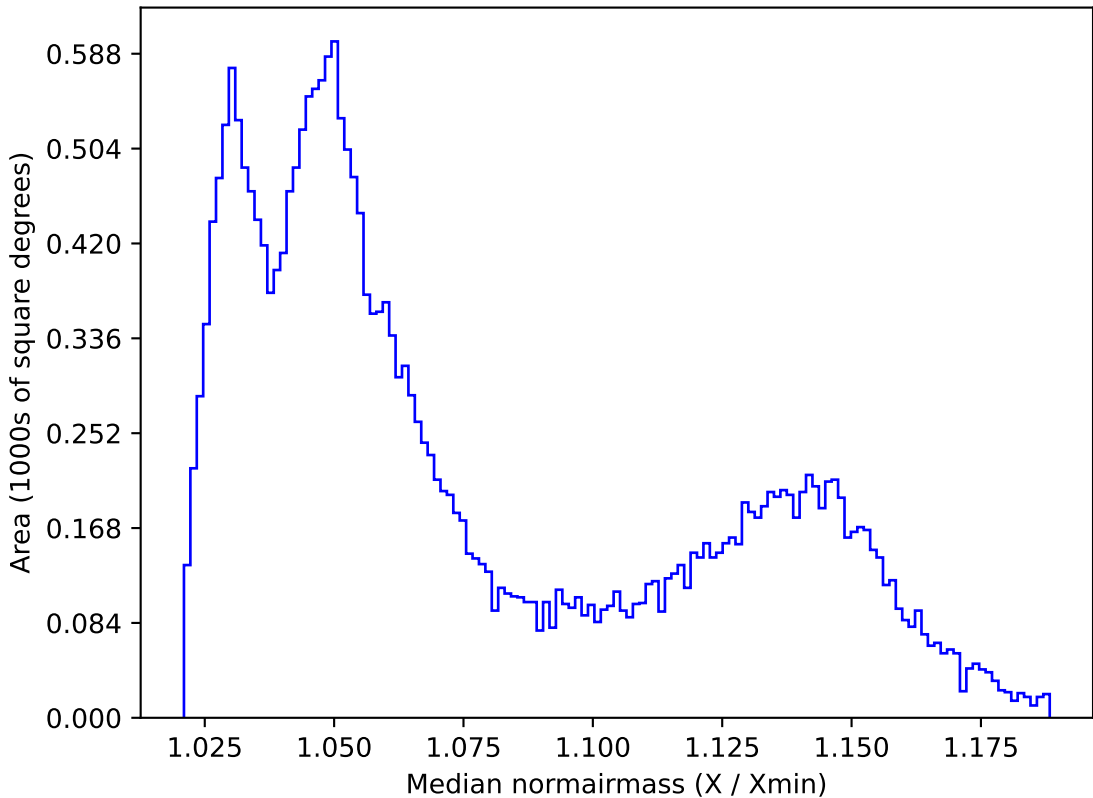
too_ignore_10_1v3.4_10yrs All sky all bands: Median normairmass
