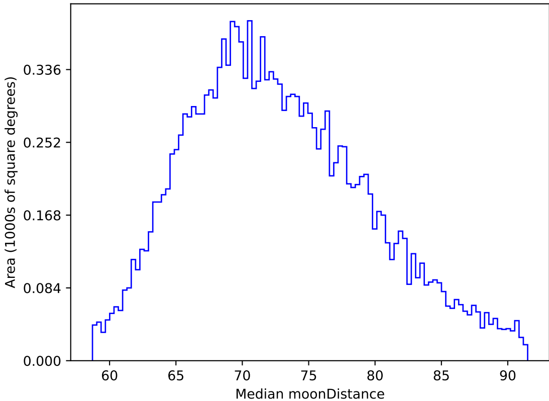
too_ignore_10_1v3.4_10yrs WFD z band: Median moonDistance
