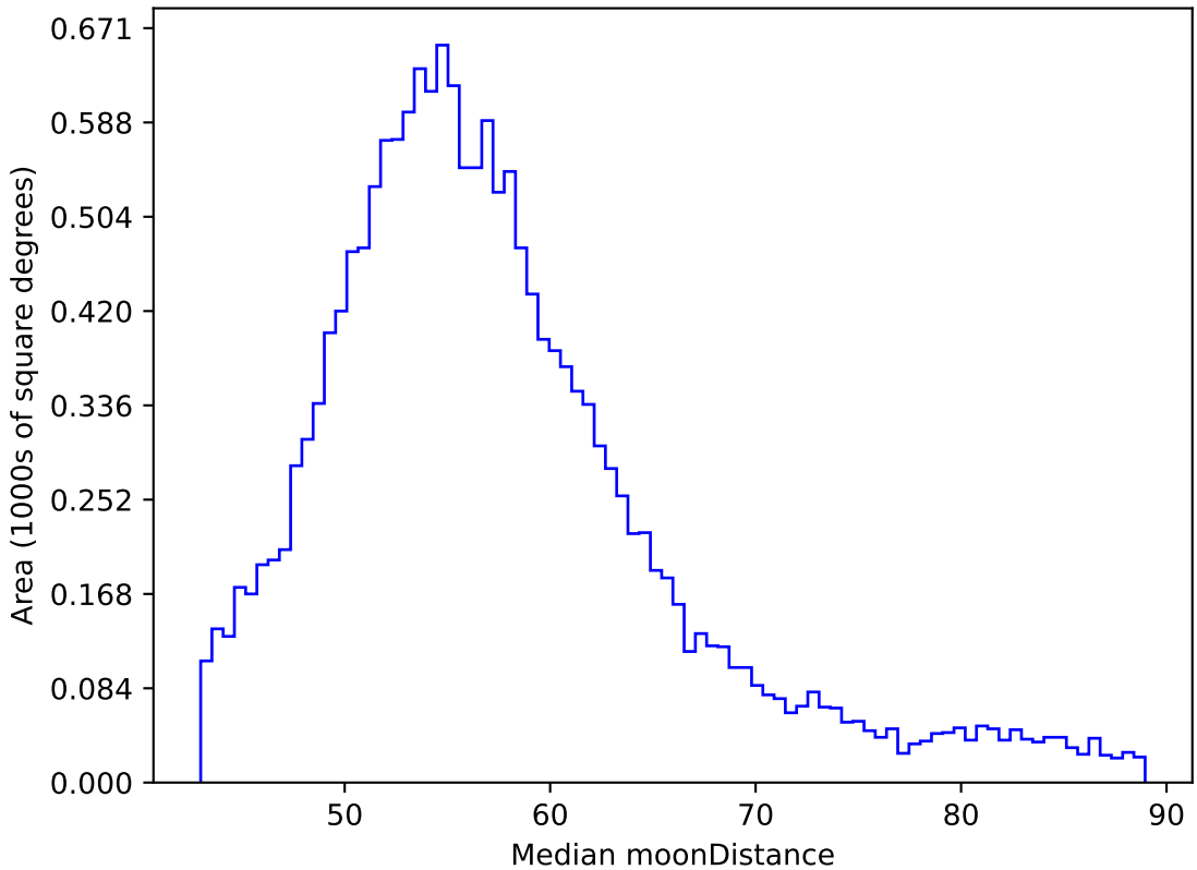
too_ignore_10_1v3.4_10yrs WFD y band: Median moonDistance
