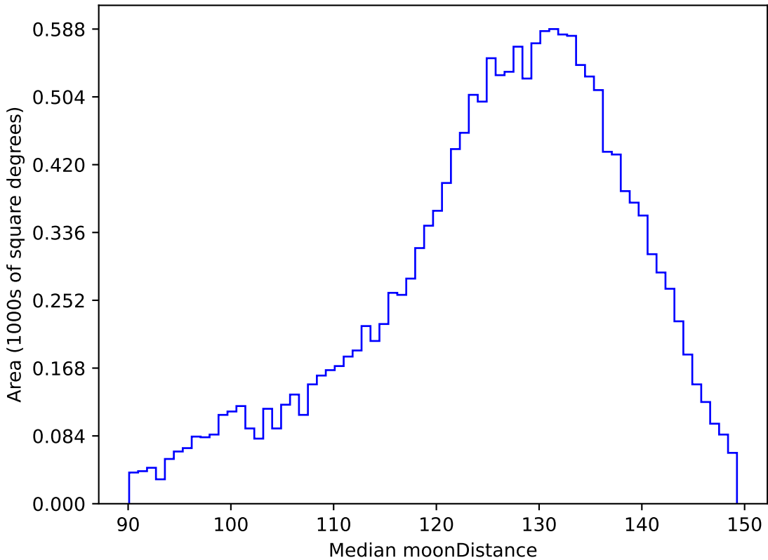
too_ignore_10_1v3.4_10yrs WFD u band: Median moonDistance
