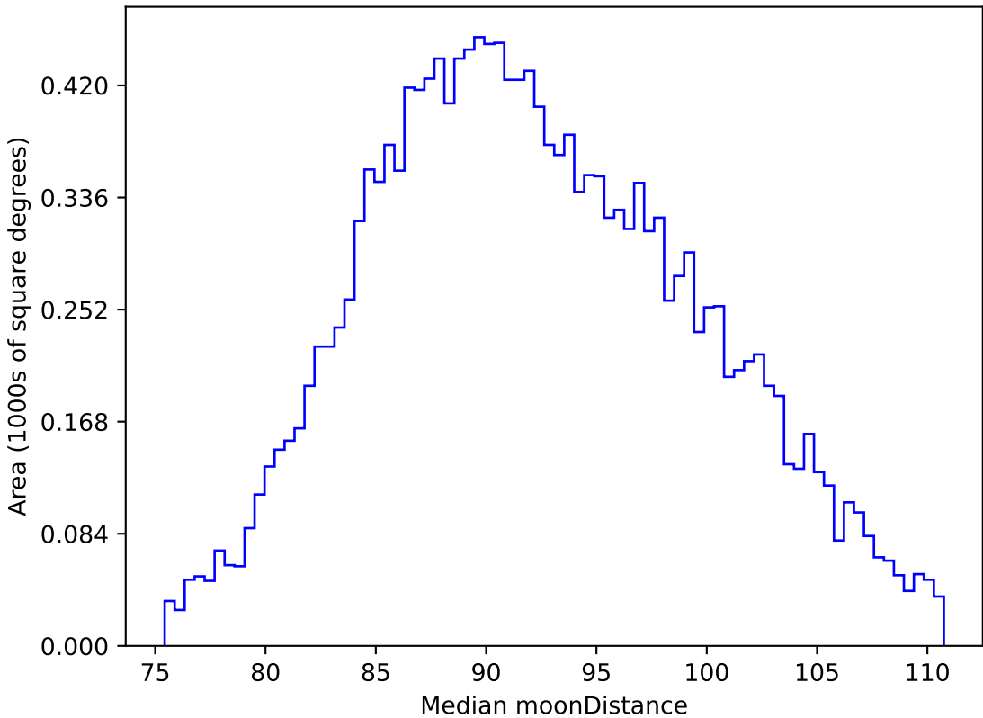
too_ignore_10_1v3.4_10yrs WFD i band: Median moonDistance
