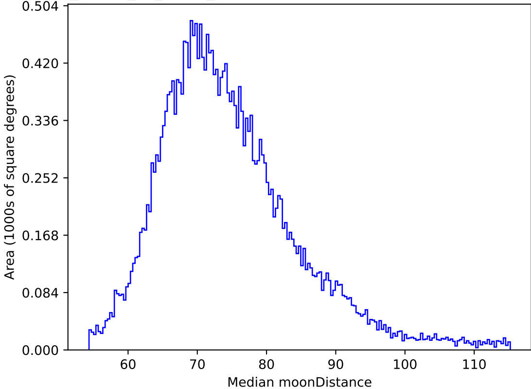
too_ignore_10_1v3.4_10yrs All sky z band: Median moonDistance
