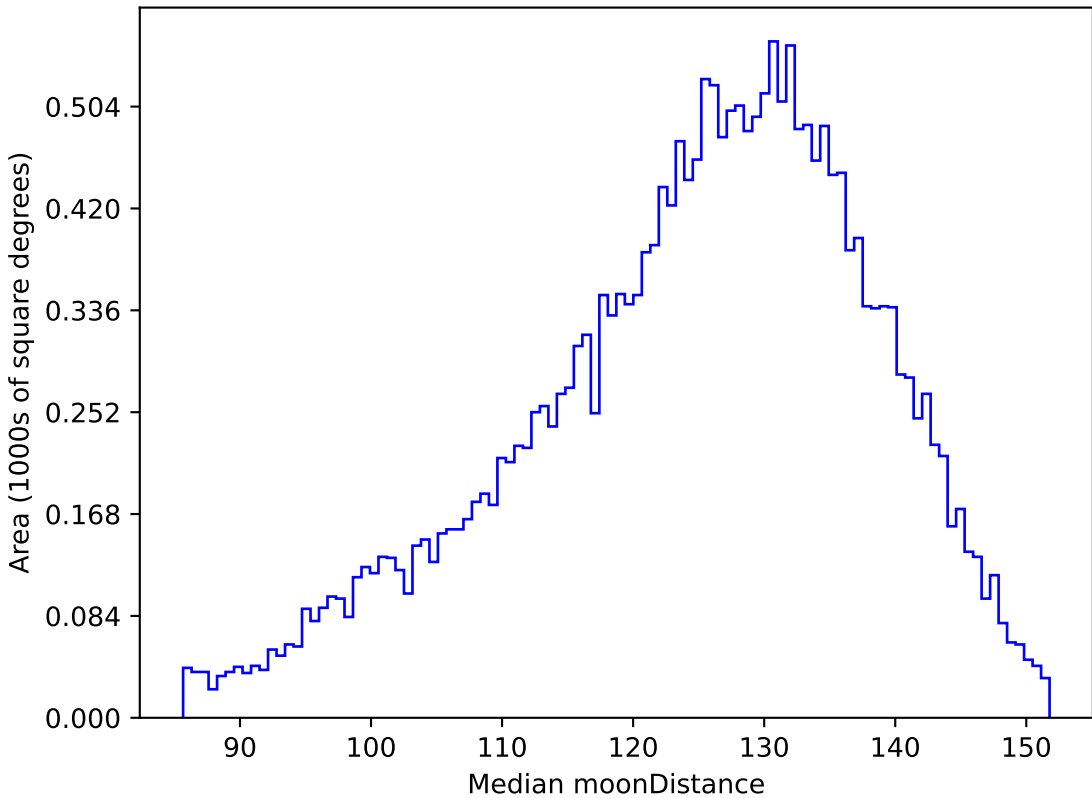
too_ignore_10_1v3.4_10yrs All sky u band: Median moonDistance
