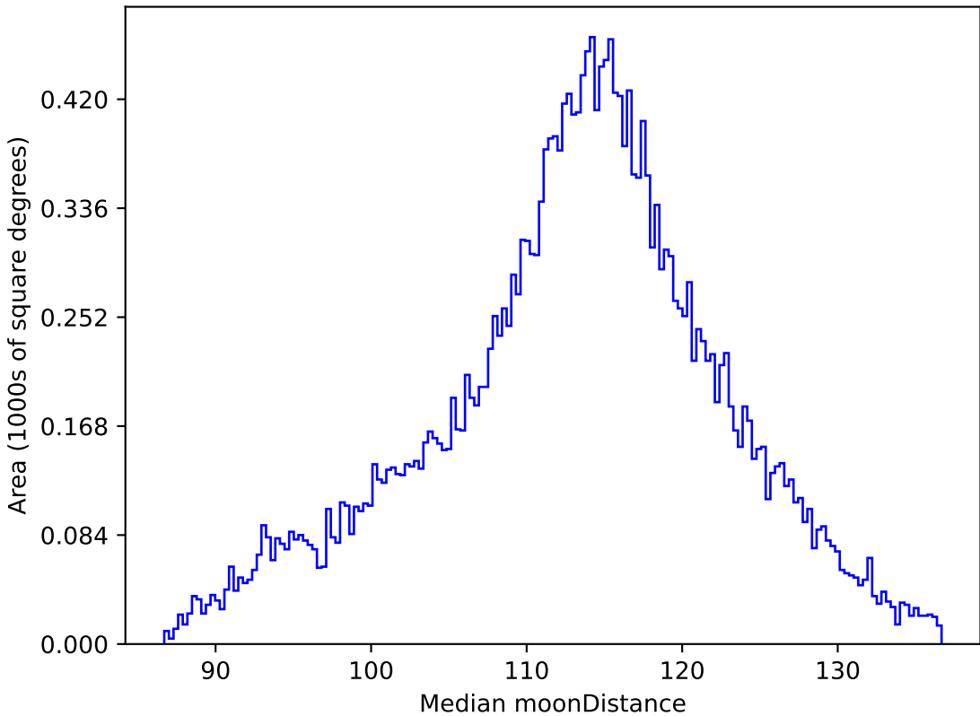
too_ignore_10_1v3.4_10yrs All sky r band: Median moonDistance
