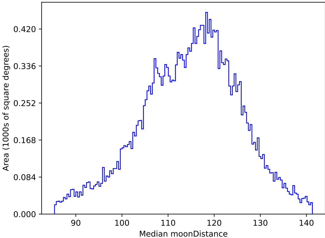
too_ignore_10_1v3.4_10yrs All sky g band: Median moonDistance
