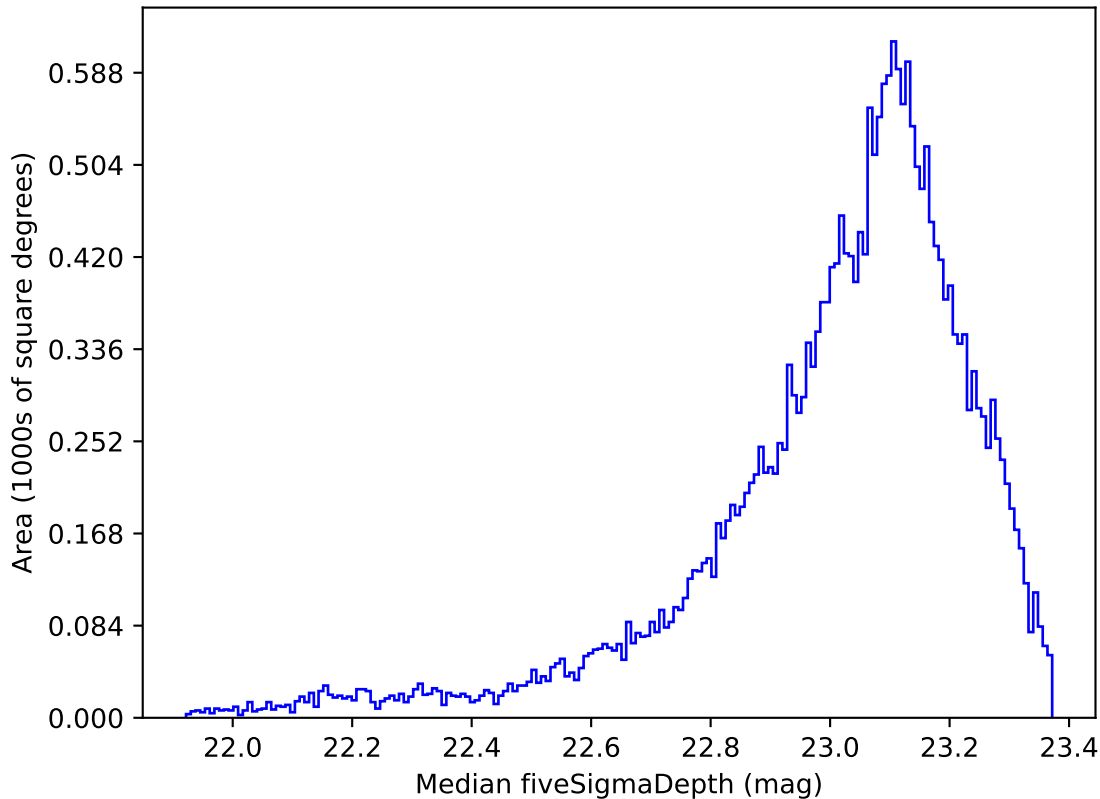
too_ignore_10_1v3.4_10yrs Yr 1 z band: Median fiveSigmaDepth
